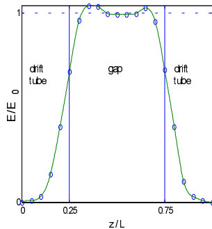
Fig. 1. The electrical field distribution along a gap
