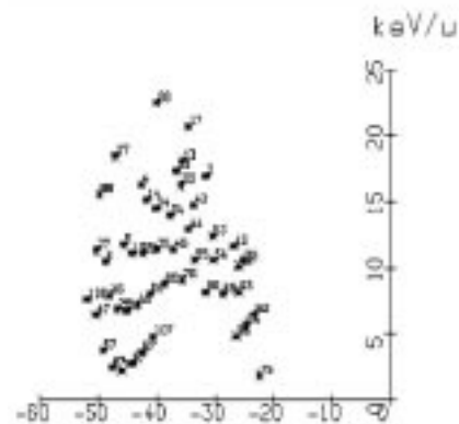
Fig.3. Bunch phase picture at the PSS-4 output.
