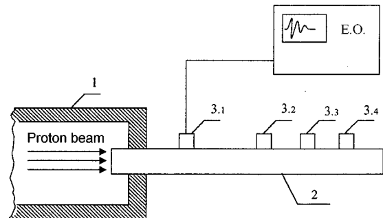
Fig. 1 Scheme of experimental setup
